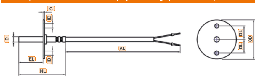
Metallic protection tube with movable polyamide flange (Construction 5)
