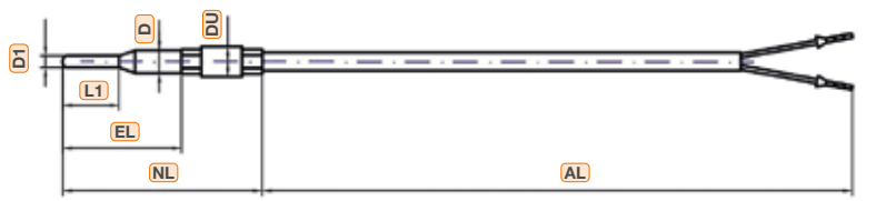
Stepped protection tube with transition sleeve on the cable
