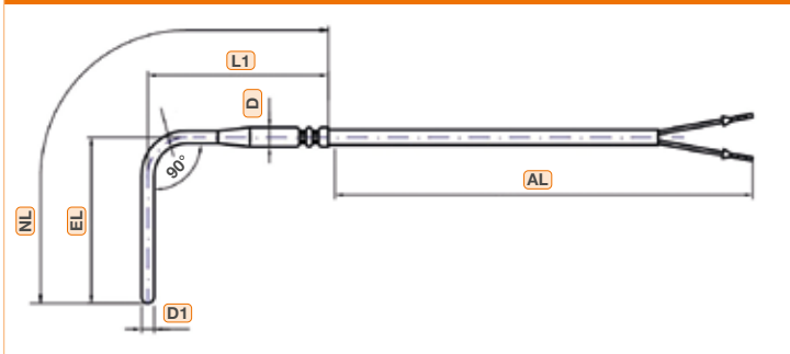
Cable temperature probe, bent and stepped protection tube
