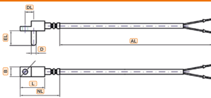
Cable temperature probe with metal surface cube with pin and mounting hole (Construction 4)
