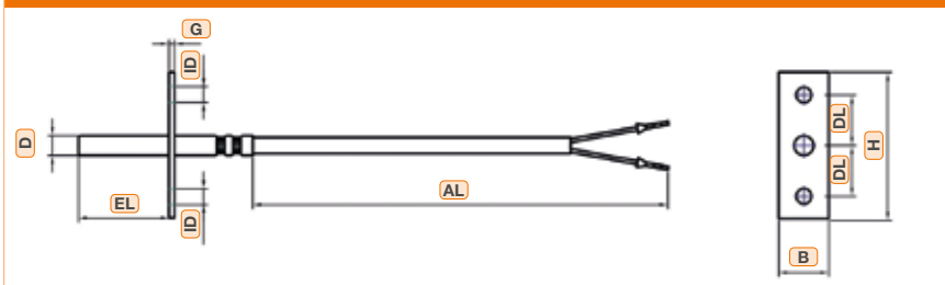
Metallic protection tube with plate and 2 mounting holes (Construction 2)
