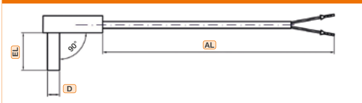
Cable temperature probe with protection tube and one-piece 90° angle connector
