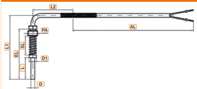
Protection tube and multiparts angle connector, loose threaded connection with spring
