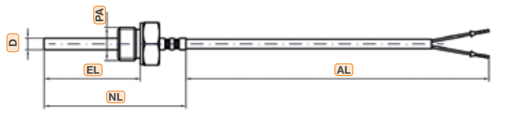
Stepped protection tube with fixed external thread
