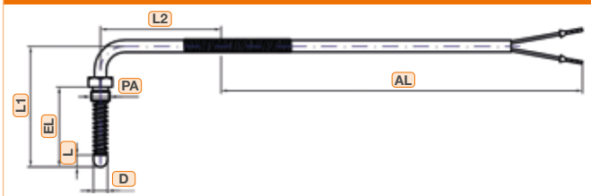
Protection tube and multiparts angle connector, loose threaded connection with spring
