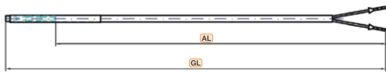
Cable temperature probe without metallic protection tube with partially exposed sensor (Construction 2)
