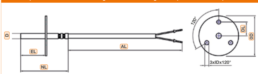
Metallic protection tube with flange and 3 mounting holes (Construction 3)
