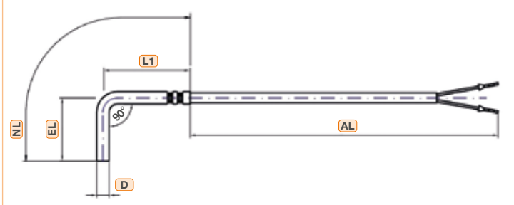
Cable temperature probe bent protection tube
