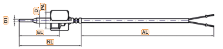
Stepped protection tube with fixed internal thread
