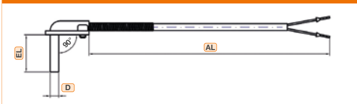
Cable temperature probe with protection tube and multipart 90° angle connector
