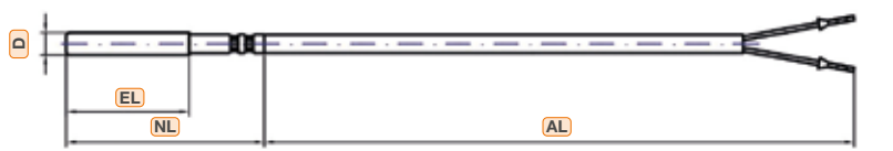
Extended protection tube (D = 8mm)
