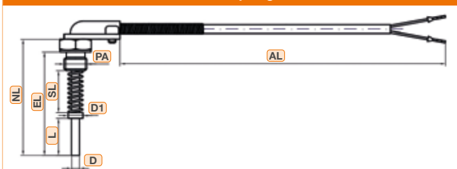
Protection tube and multiparts angle connector, loose threaded connection with spring
