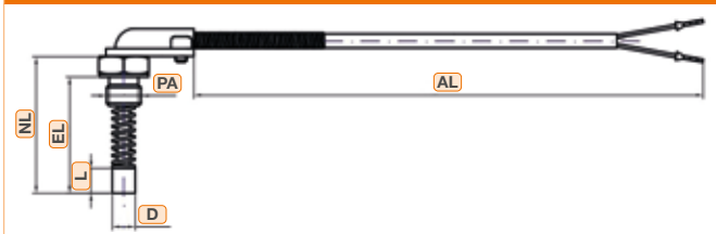
Bent protection tube and loose threaded connection with spring
