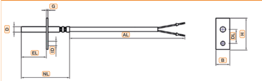
Metallic protection tube with plate and 1 mounting hole (Construction 1)
