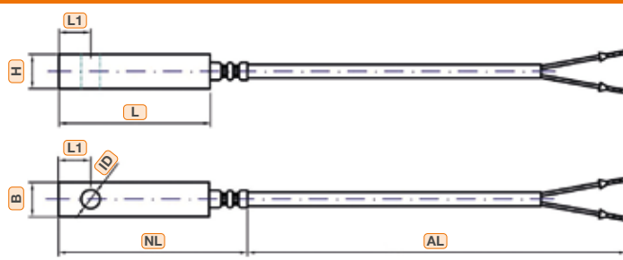
Cable temperature probe with metal surface cube with mounting hole (Construction 2)
