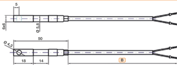
Cable temperature probe with universal metal surface cube with mounting hole and /or for band mounting (Construction 1)
